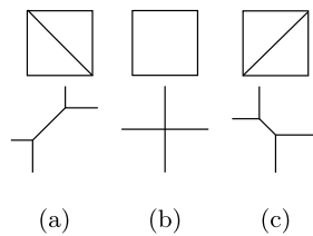
FIGURE 10.—All possible demand complexes, and examples of their dual weighted LIPs, giving all the combinatorial types when \mathcal{A} = \{0, 1\}^2 .
