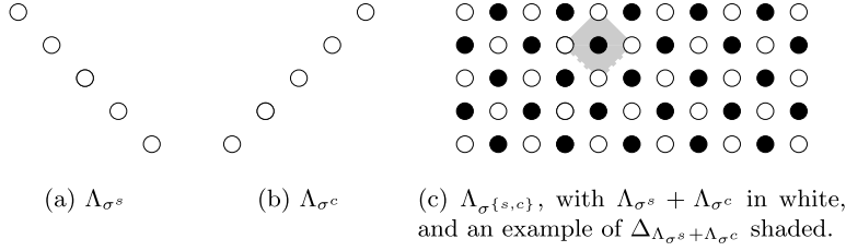
FIGURE 9.—The parallel lattices corresponding to demand complex cells \sigma^s , \sigma^c , and \sigma^{[s,c]} of, respectively, u^s , u^c , and u^{[s,c]} (as shown in Figures 4(a)–(c) and Figures 5(a)–(c)) at \mathbf{p} = (30, 20) .
