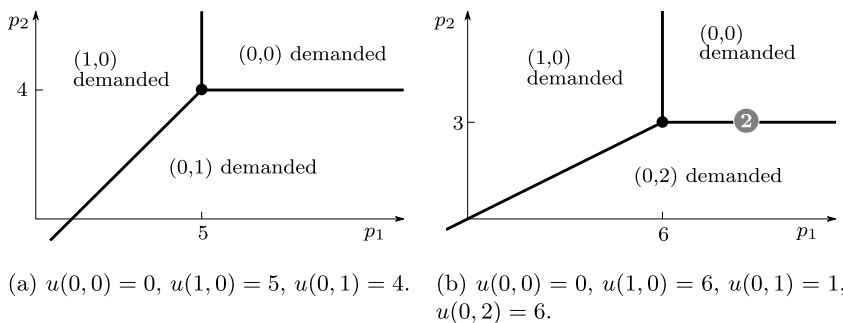
FIGURE 1.—Examples of LIPs, \mathcal{L}_u , for two valuations, u . The facets are the line segments; the labeled facet in (b) has weight 2. The bundle demanded in each UDR is labeled.
